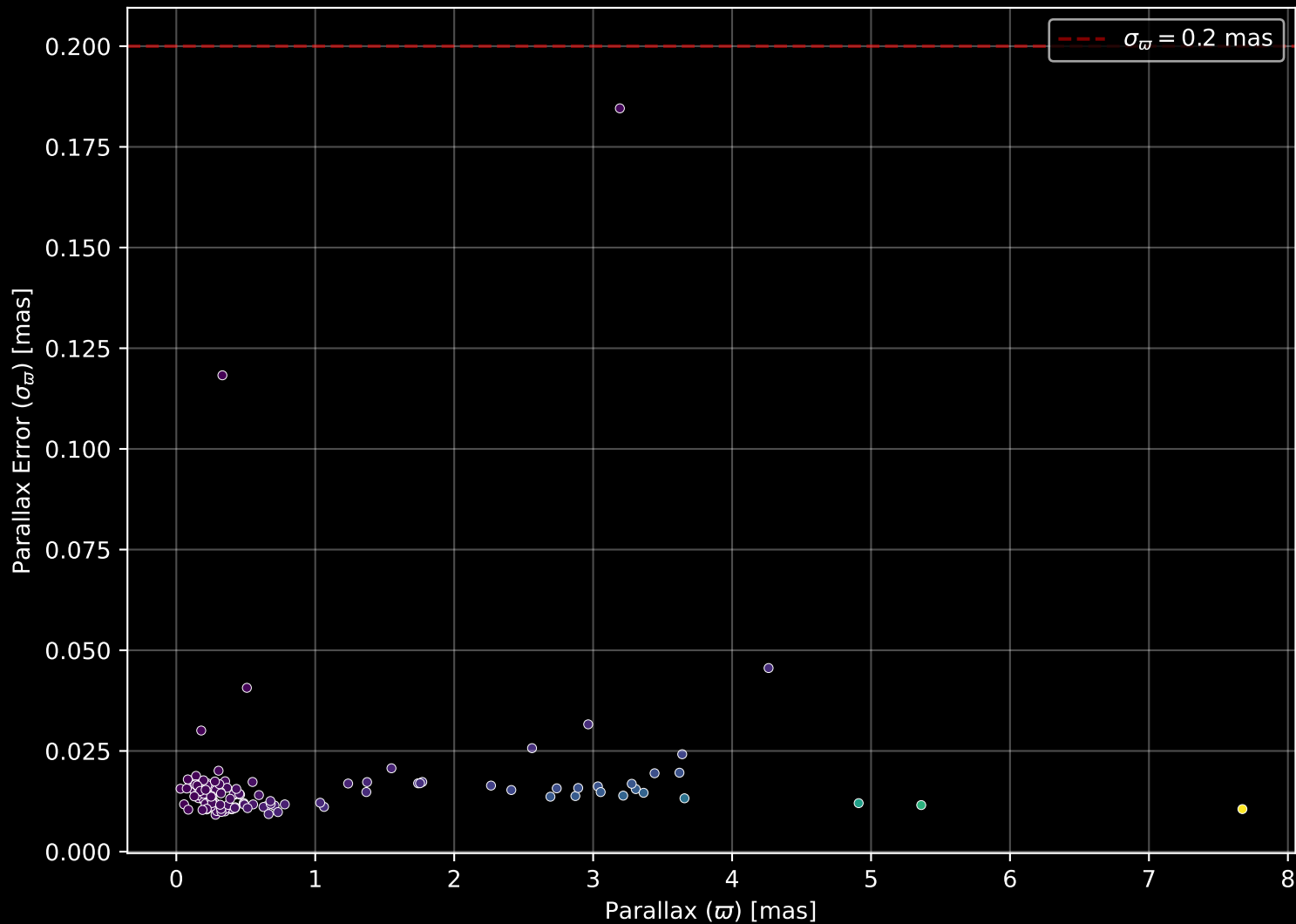
APOGEE DR17 Field: [060+12] Parallax Quality (n= 140)
