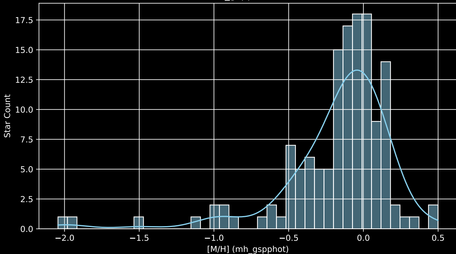
APOGEE DR17 Field: [060+12 [M/H] (mh_gspphot) (n= 138)
