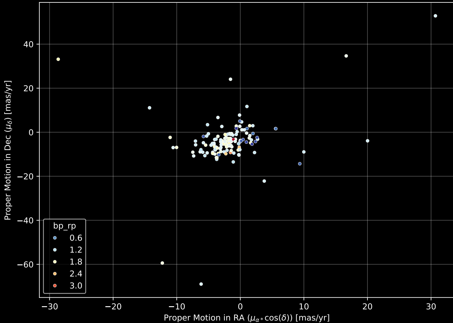
APOGEE DR17 Field: [060+12] Proper Motion Diagram (n= 140)
