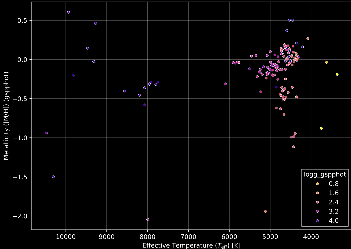
APOGEE DR17 Field: [060+12] Stellar Population Parameters (n= 140)
