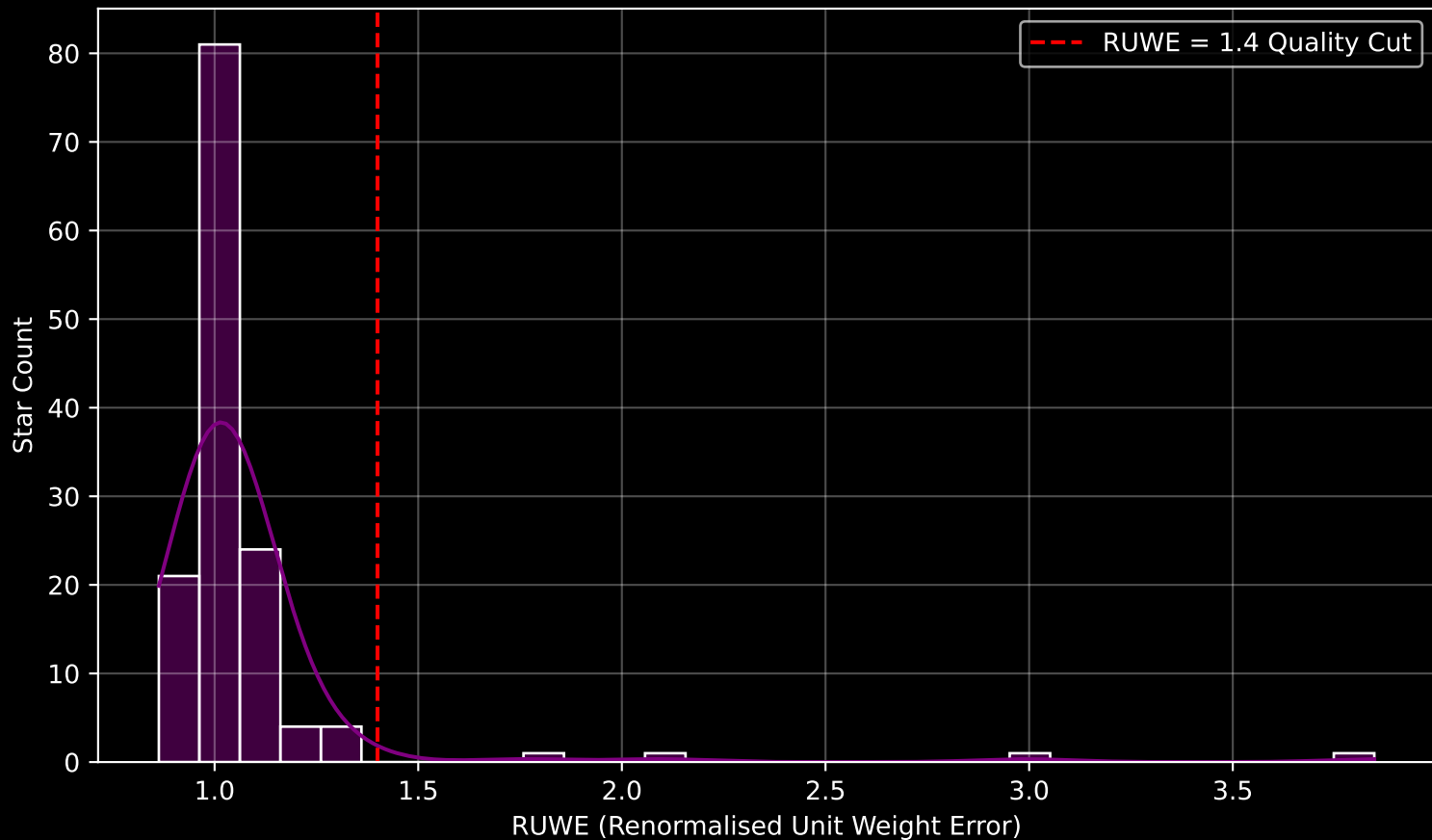
GAPOGEE DR17 Field [060+12] RUWE Distribution (n= 138)
